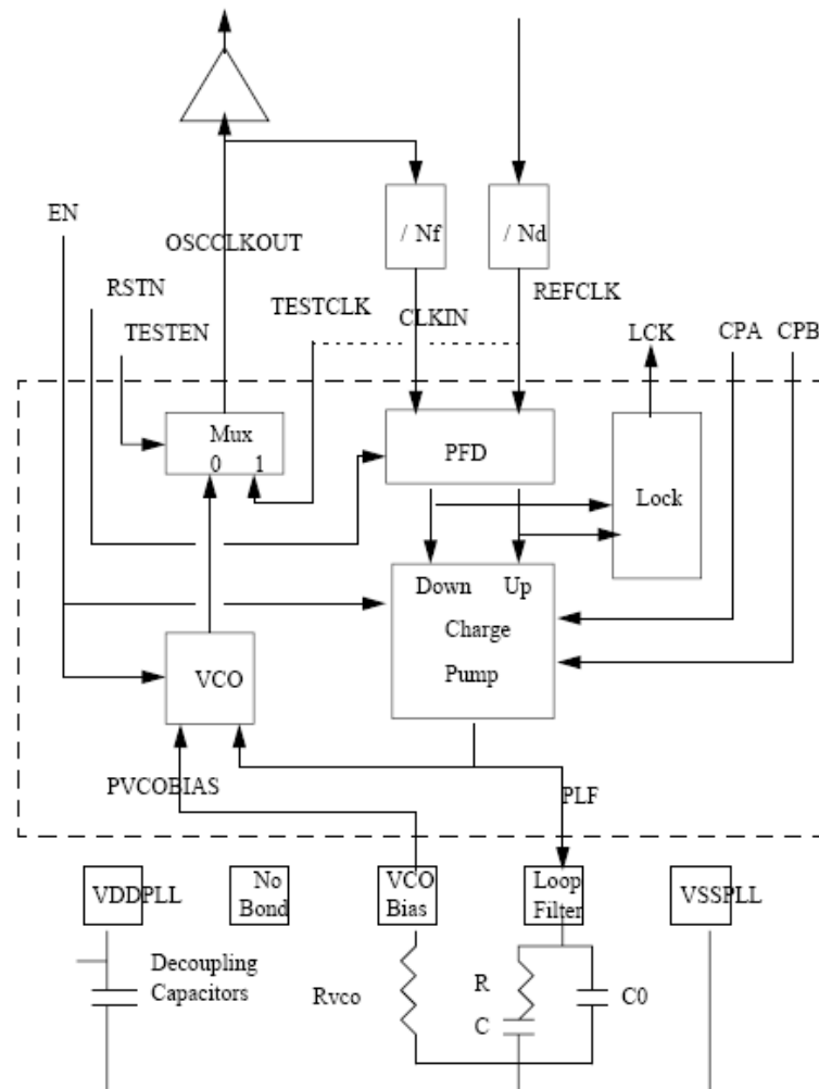
Figure 5-3 PLL with external components
