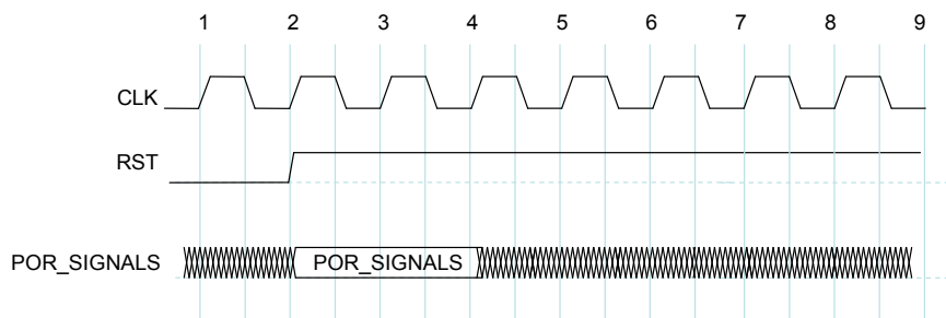
Figure 6-7 Reset configuration interface timing specification
