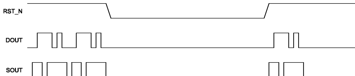
Figure 13-1 Reset Waveform
