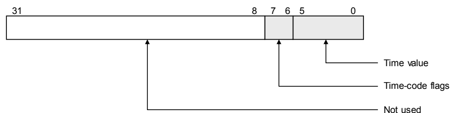
Figure 9-7 Time-Code Register Fields
