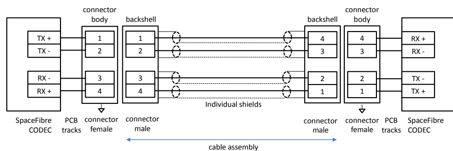
Figure 5-14 SpaceFibre flight cable assembly
