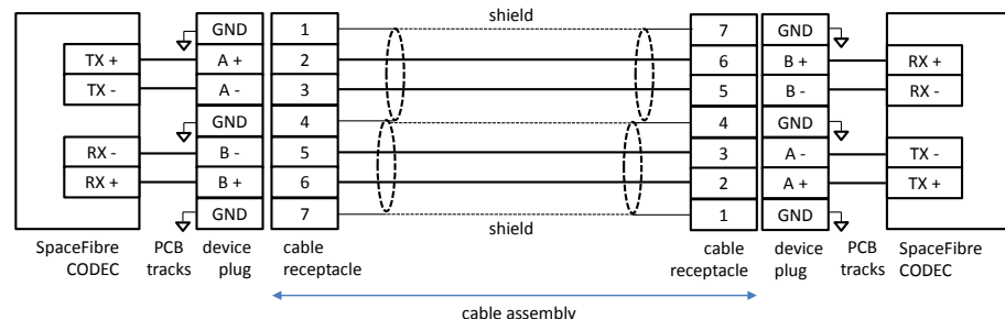
Figure 5-13 SpaceFibre EGSE cable assembly
