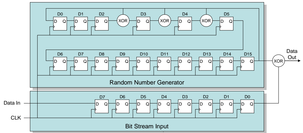
Figure A-1 Scrambler / De-Scrambler
