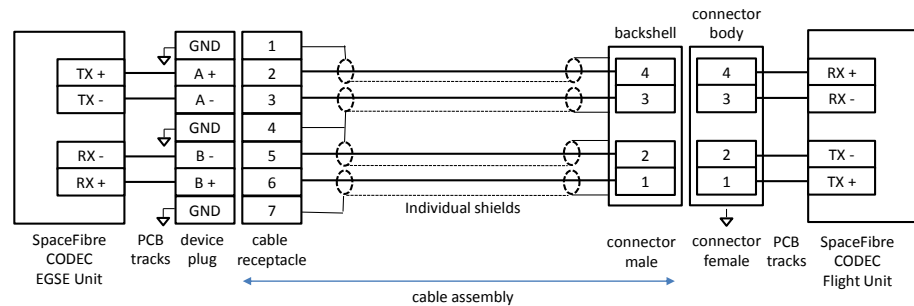
Figure 5-15 SpaceFibre EGSE to flight adaptor cable assembly
